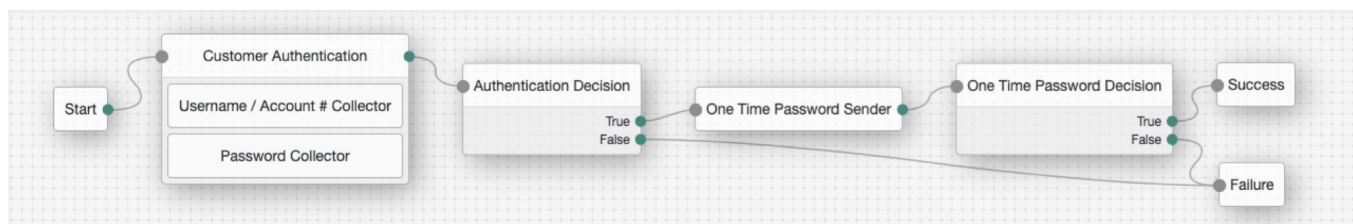
One Time Password Tree
